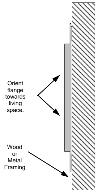
Side view of pre-construction bracket.
