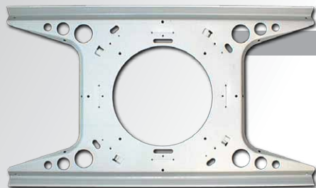
PB-6 & PB-8 Formed sheet metal T-bar bridge to reinforce T-bar drop ceilings for installation of all 8" & 6-1/2" round speakers with snap in PE-8 Plenum Dome (shown below) for Fire Rated applications.
