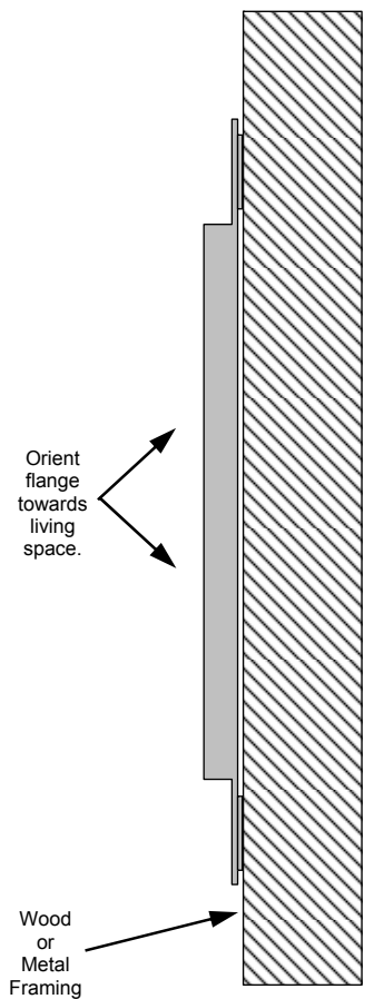
Side view of pre-construction bracket.
